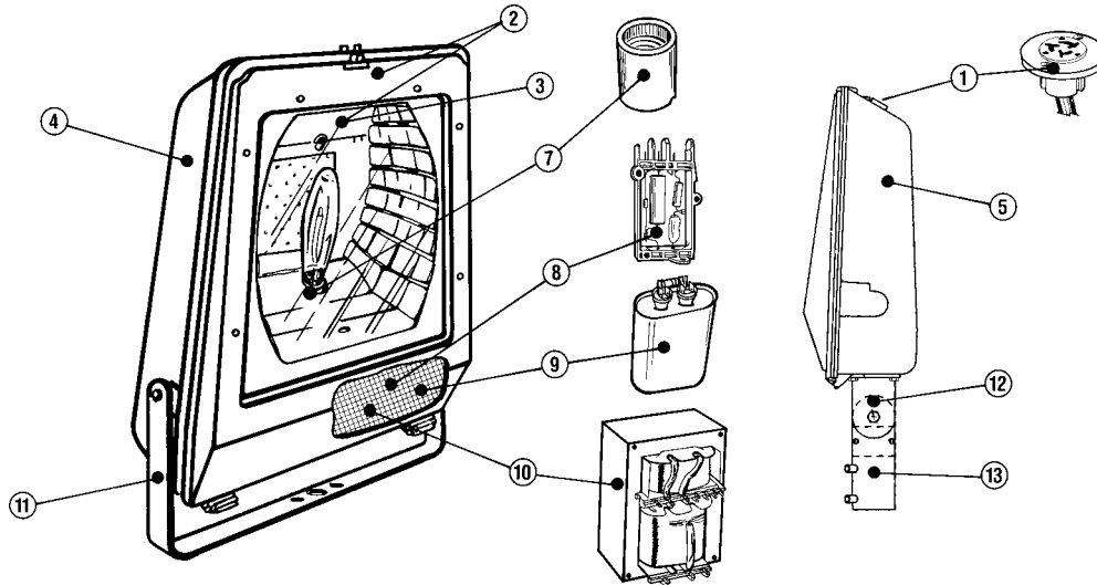
GLAREFIGHTER™ ASYMMETRIC FLOODLIGHT
